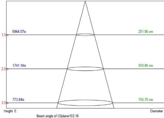
PHX22-145-5K-U Lux Distance Curve
