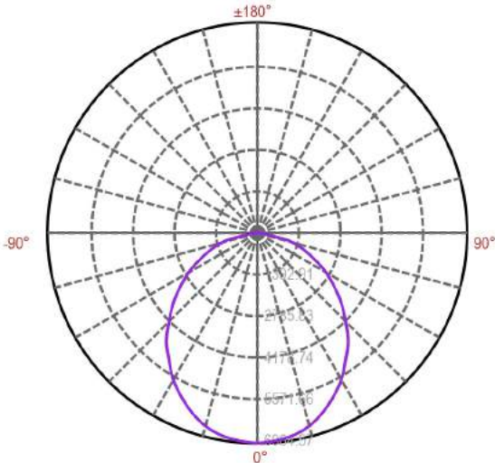
PHX22-145-5K-U Light Distribution Curve [Unit: CD]
