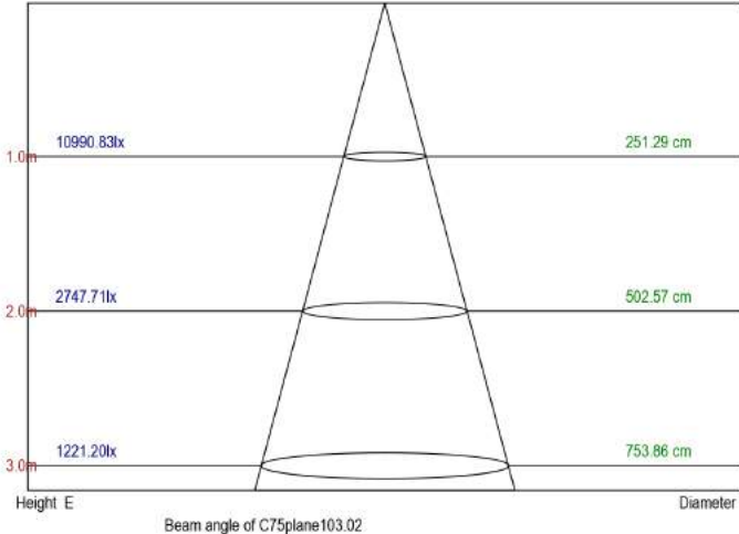
PHX22-230-5K-U Lux Distance Curve
