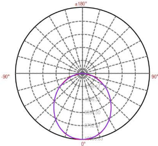
PHX22-230-5K-U Light Distribution Curve [Unit: CD]
