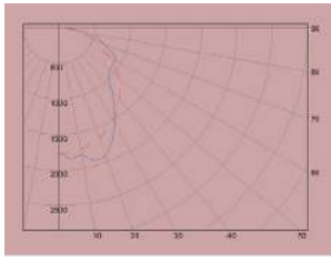
0° Candela Plot 45° 2 Lamp T8 90°
